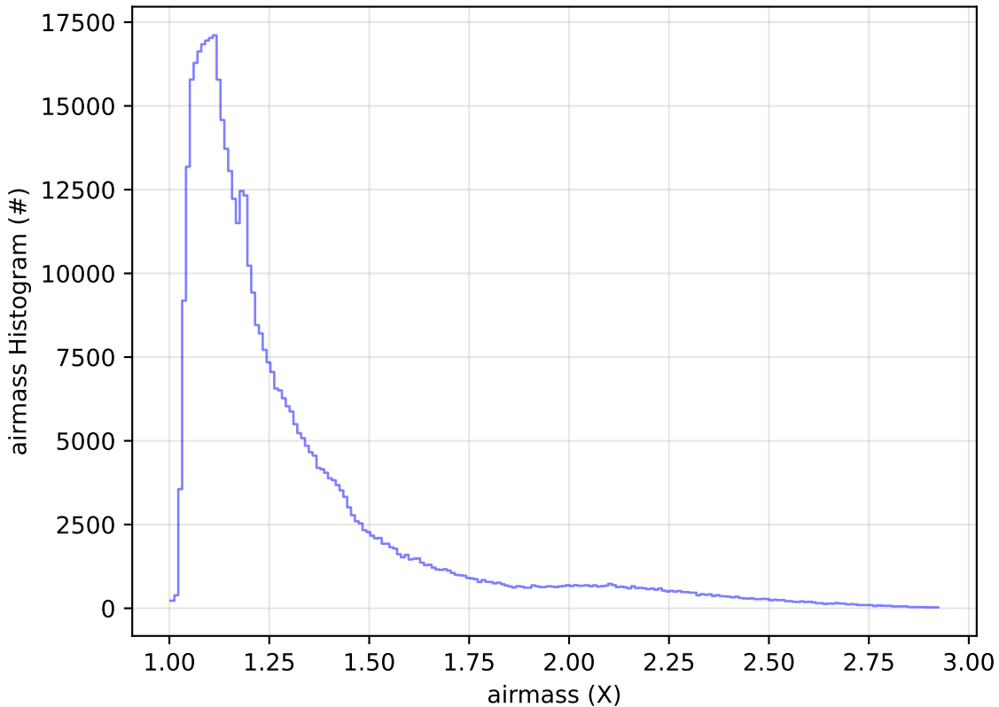
ddf_acor_sf10_lsf15_lsr10_v3.4_10yrs All sky i band: airmass Histogram
