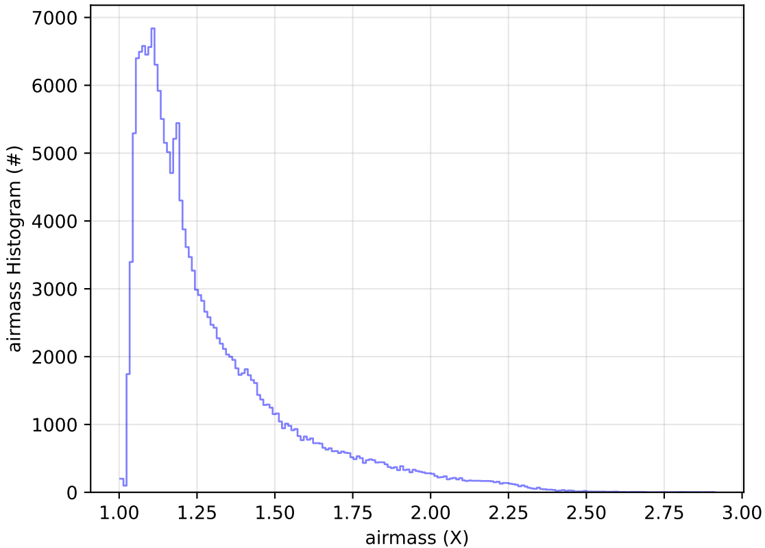
ddf_acor_sf10_lsf15_lsr10_v3.4_10yrs All sky g band: airmass Histogram
