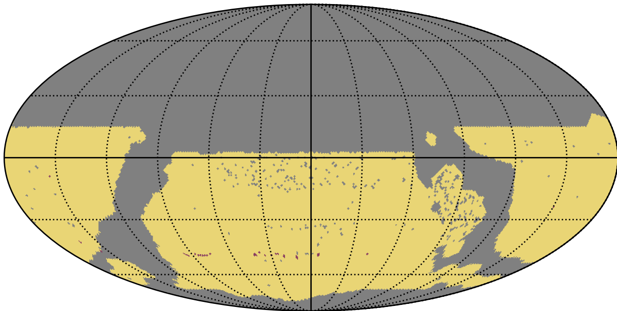
ddf_acor_sf10_lsf15_lsr10_v3.4_10yrs WFD: RapidRevisits
