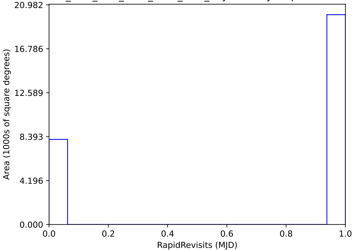
ddf_acor_sf10_lsf15_lsr10_v3.4_10yrs All sky: RapidRevisits
