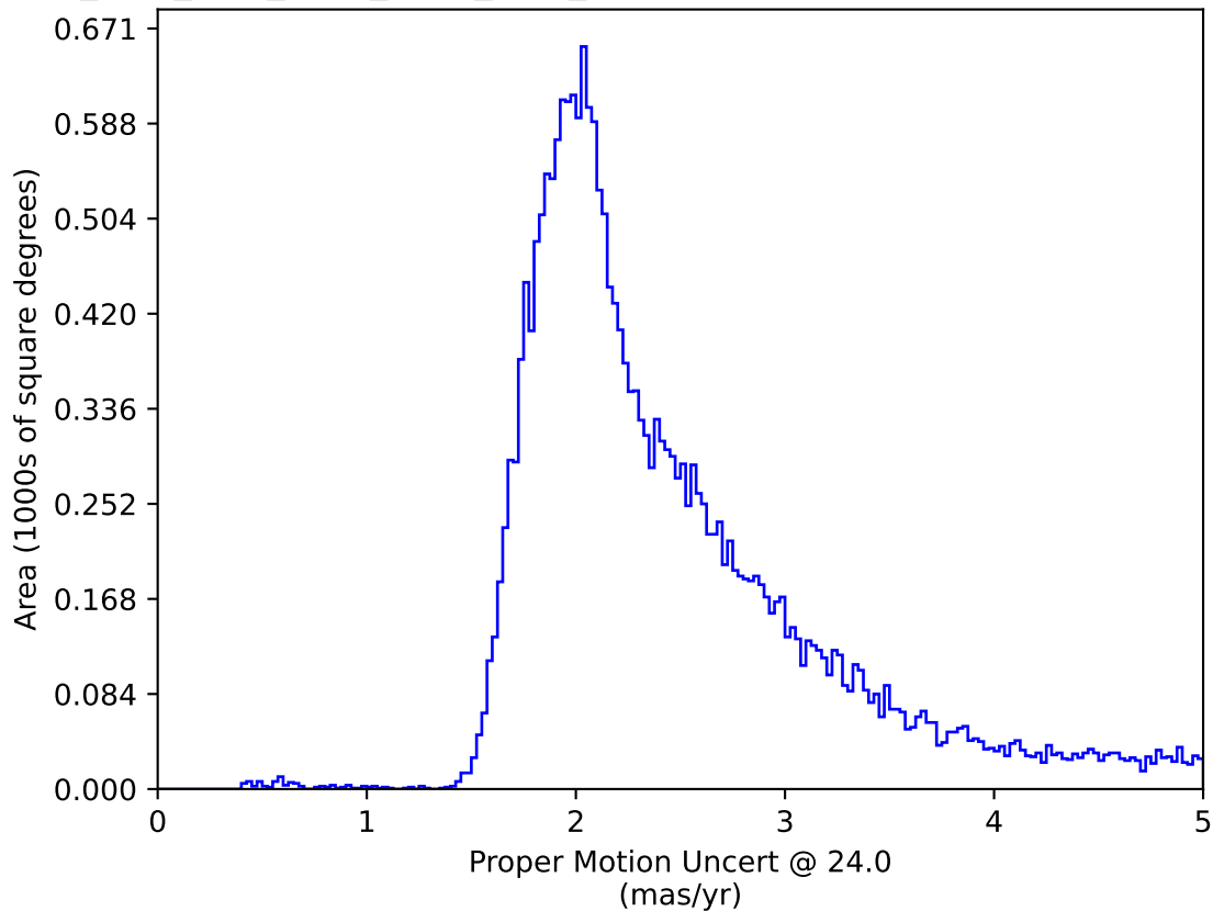
ddf_acor_sf10_lsf15_lsr10_v3.4_10yrs All sky: Proper Motion Uncert @ 24.0
