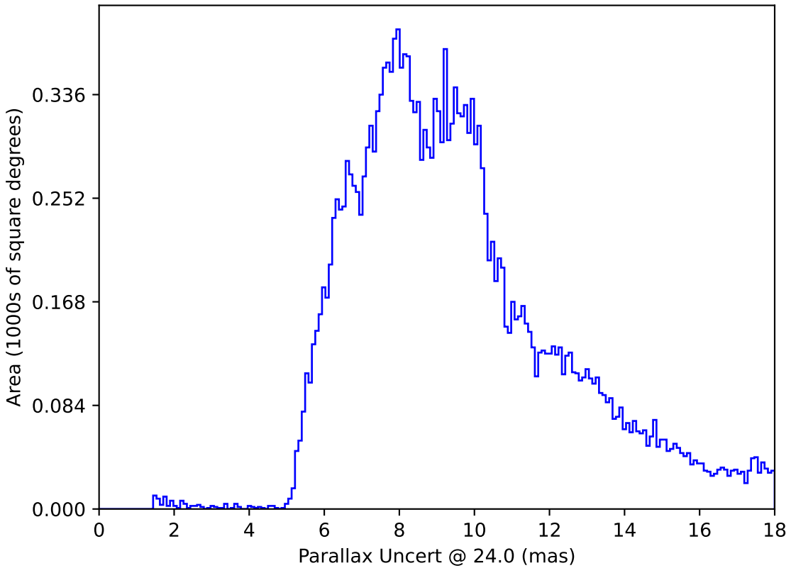
ddf_acor_sf10_lsf15_lsr10_v3.4_10yrs All sky: Parallax Uncert @ 24.0
