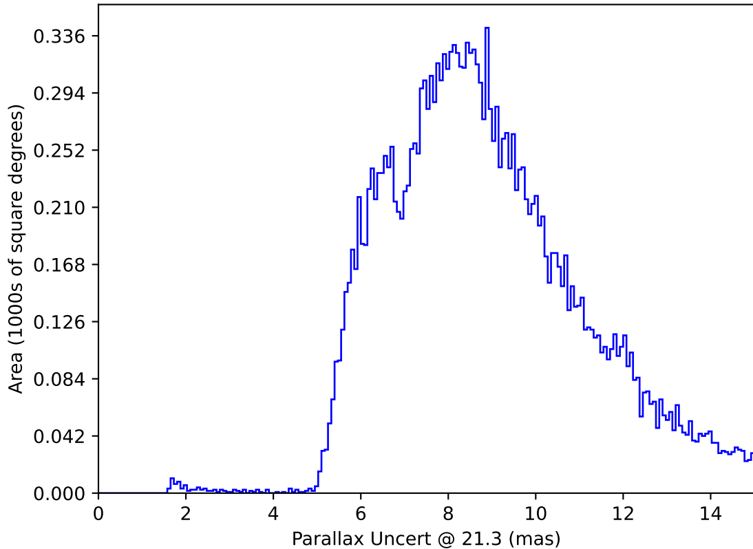
ddf_acor_sf10_lsf15_lsr10_v3.4_10yrs All sky y band only: Parallax Uncert @ 21.3
