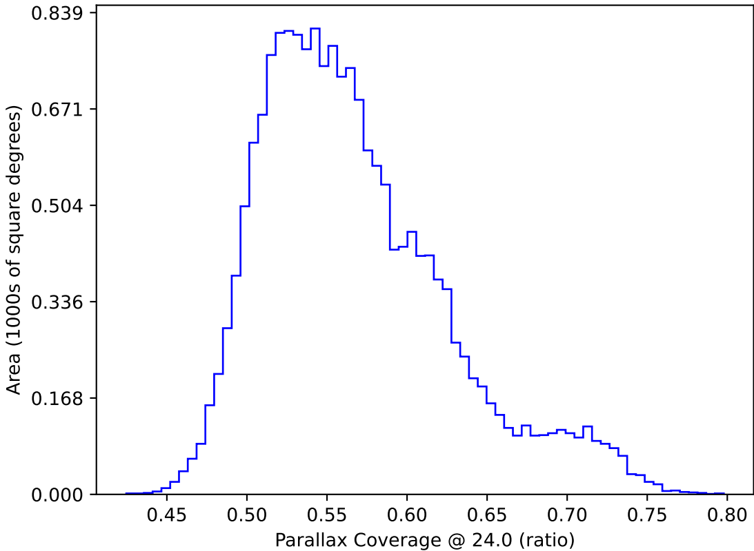
ddf_acor_sf10_lsf15_lsr10_v3.4_10yrs WFD: Parallax Coverage @ 24.0
