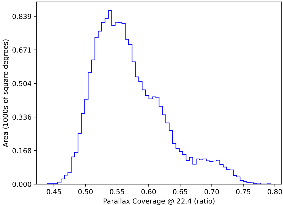
ddf_acor_sf10_lsf15_lsr10_v3.4_10yrs WFD: Parallax Coverage @ 22.4
