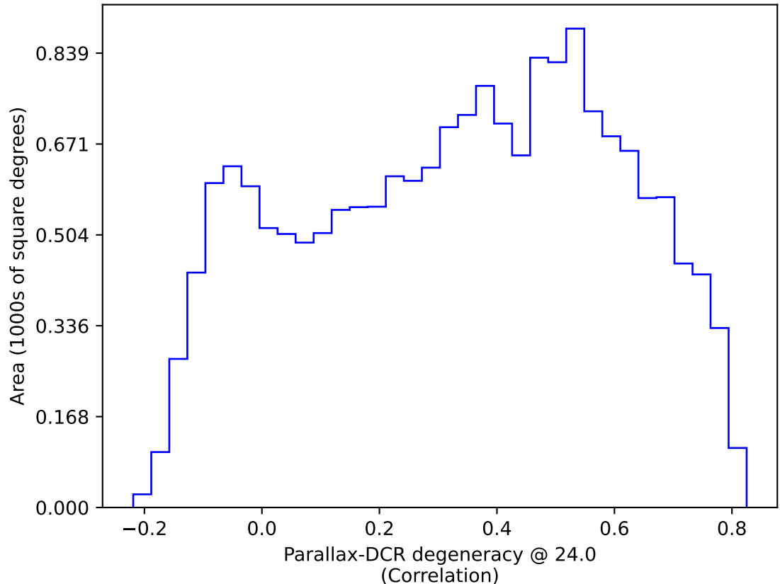
ddf_acor_sf10_ls15_lsr10_v3.4_10yrs WFD: Parallax-DCR degeneracy @ 24.0
