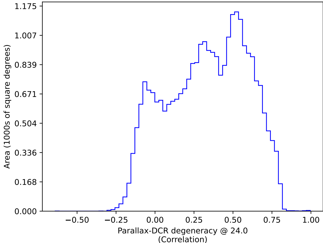
ddf_acor_sf10_lsf15_lsr10_v3.4_10yrs All sky: Parallax-DCR degeneracy @ 24.0
