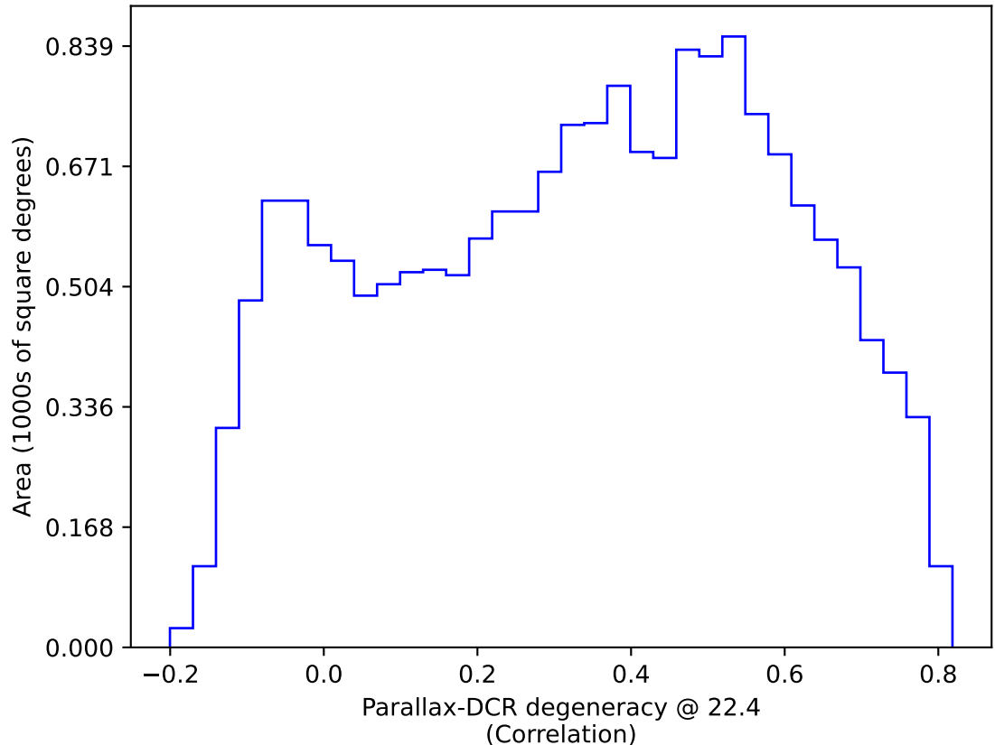
ddf_acor_sf10_lsf15_lsr10_v3.4_10yrs WFD: Parallax-DCR degeneracy @ 22.4
