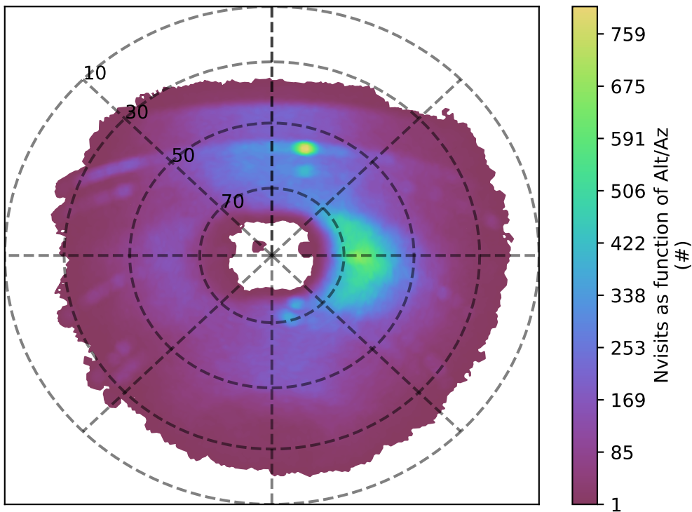
ddf_acor_sf10_ls15_lsr10_v3.4_10yrs u band: Nvisits as function of Alt/Az
