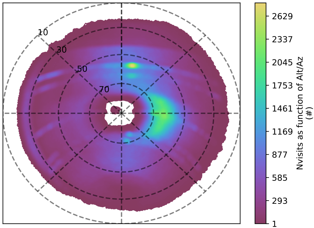
ddf_acor_sf10_lsf15_lsr10_v3.4_10yrs r band: Nvisits as function of Alt/Az
