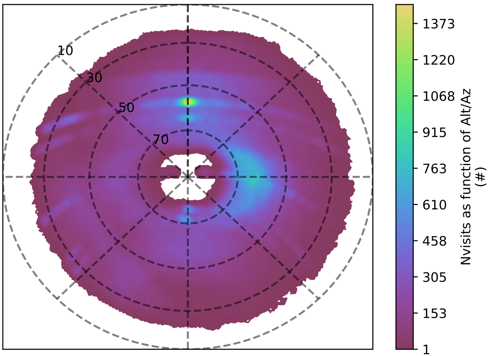
ddf_acor_sf10_lsf15_lsr10_v3.4_10yrs g band: Nvisits as function of Alt/Az
