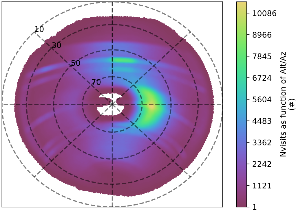
ddf_acor_sf10_ls15_lsr10_v3.4_10yrs all bands: Nvisits as function of Alt/Az
