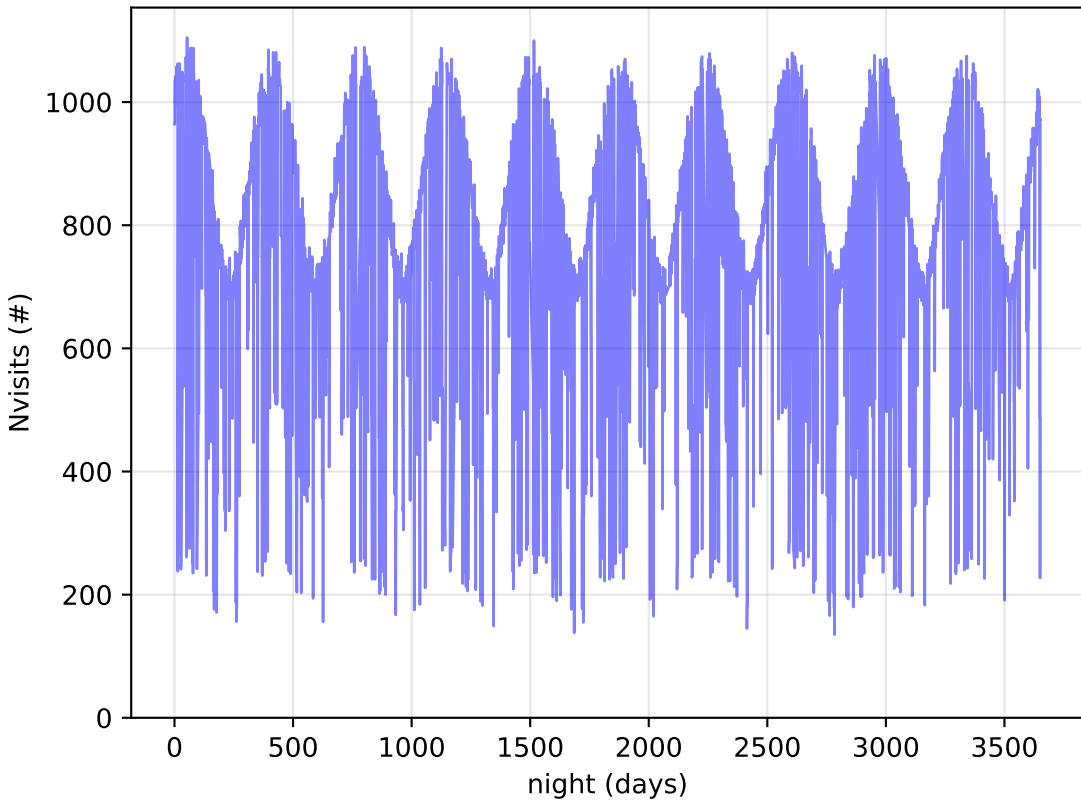
ddf_acor_sf10_ls15_lsr10_v3.4_10yrs All visits: Nvisits
