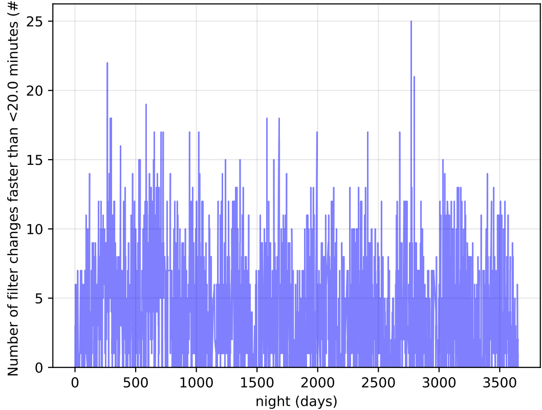
ddf_acor_sf10_Isf15_Isr10_v3.4_10yrs Per Night: Number of filter changes faster than <20.0 minutes
