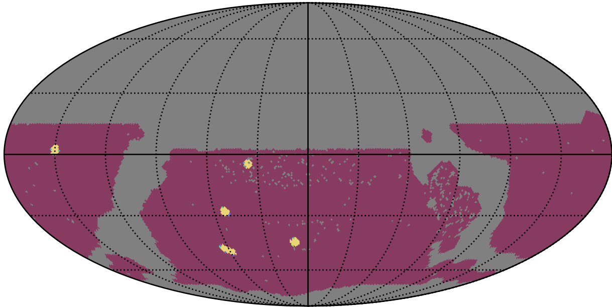
ddf_acor_sf10_lsf15_lsr10_v3.4_10yrs WFD: NumberOfQuickRevisits
