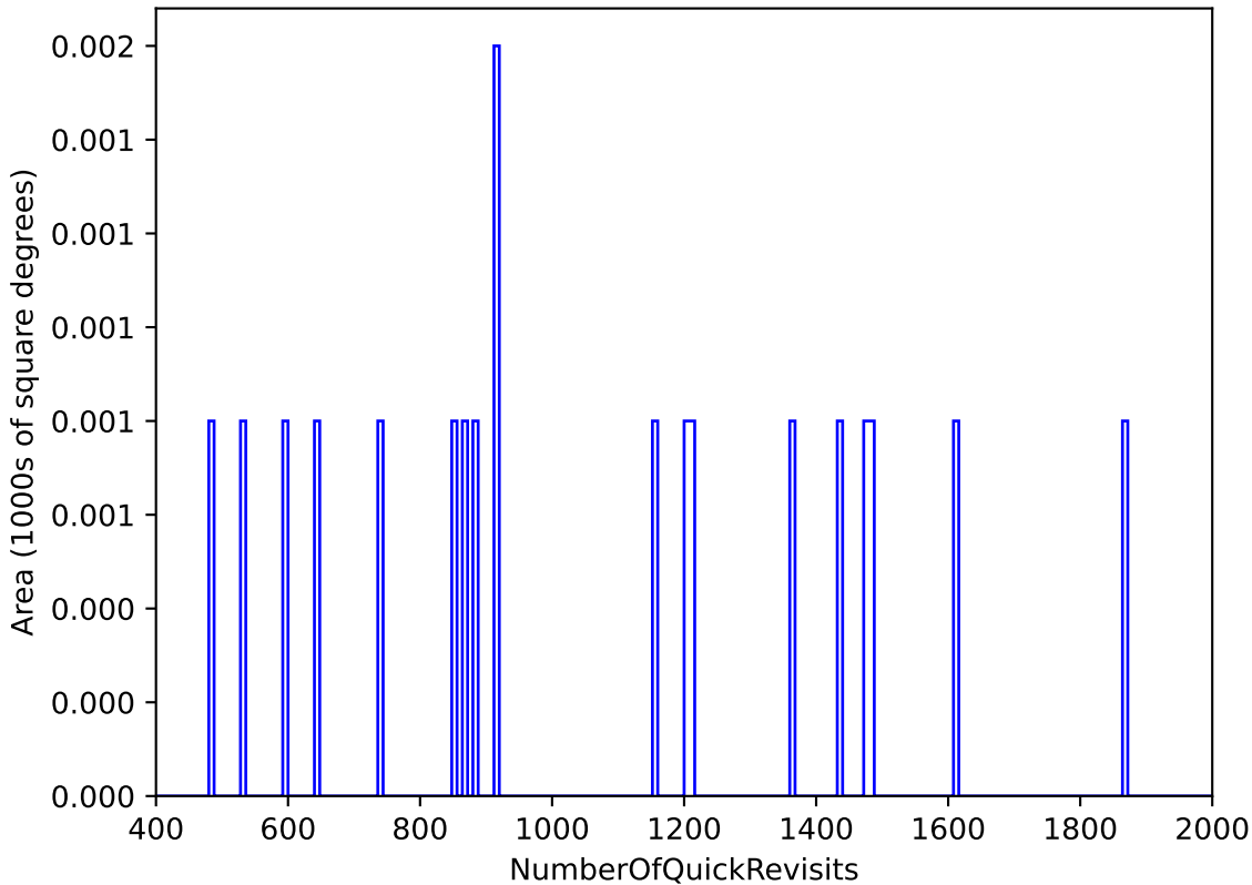
ddf_acor_sf10_lsf15_lsr10_v3.4_10yrs All sky: NumberOfQuickRevisits
