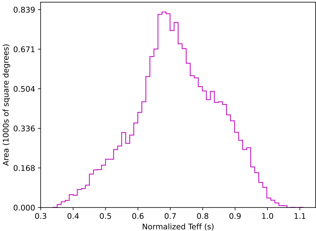
ddf_acor_sf10_lsf15_lsr10_v3.4_10yrs WFD z band: Normalized Teff
