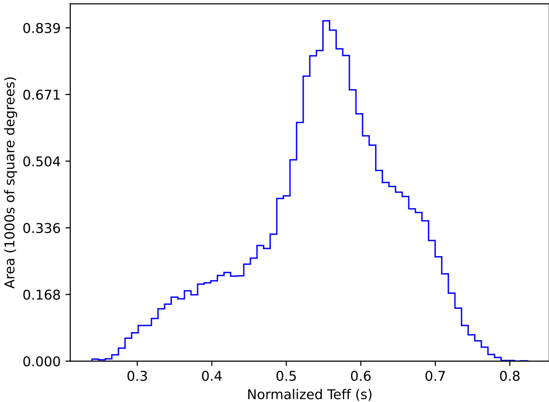
ddf_acor_sf10_lsf15_lsr10_v3.4_10yrs WFD y band: Normalized Teff
