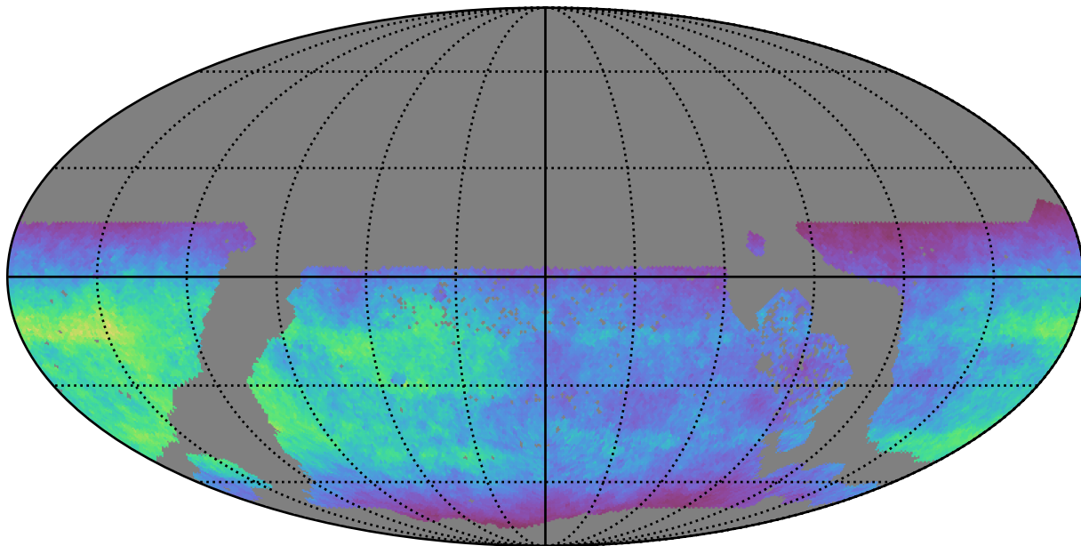
ddf_acor_sf10_lsf15_lsr10_v3.4_10yrs WFD u band: Normalized Teff
