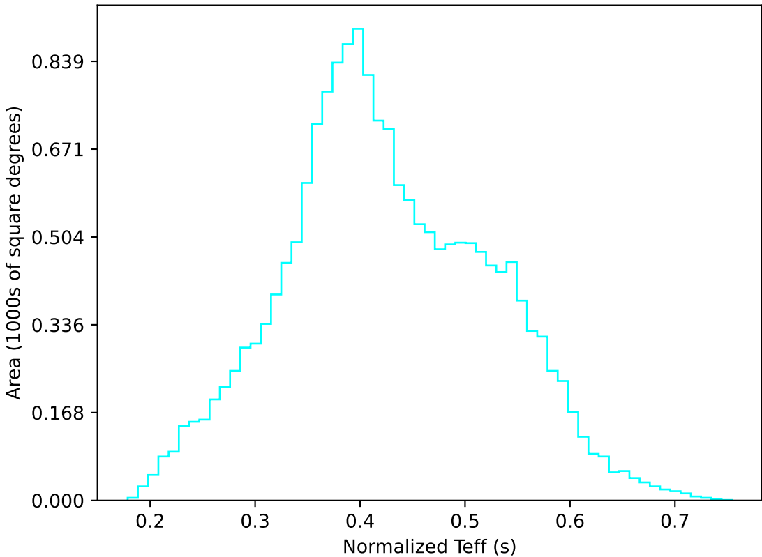
ddf_acor_sf10_lsf15_lsr10_v3.4_10yrs WFD u band: Normalized Teff
