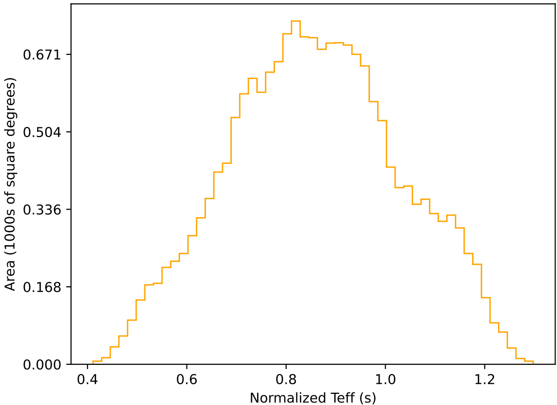
ddf_acor_sf10_lsf15_lsr10_v3.4_10yrs WFD r band: Normalized Teff
