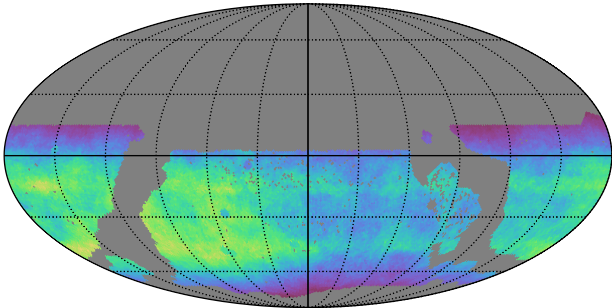
ddf_acor_sf10_lsf15_lsr10_v3.4_10yrs WFD i band: Normalized Teff
