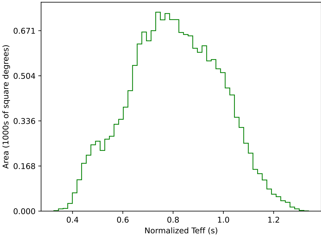
ddf_acor_sf10_ls15_lsr10_v3.4_10yrs WFD g band: Normalized Teff
