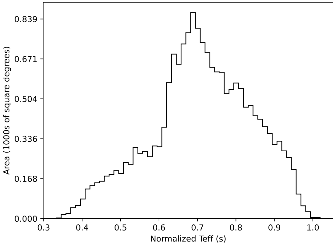
ddf_acor_sf10_lsf15_lsr10_v3.4_10yrs WFD all bands: Normalized Teff
