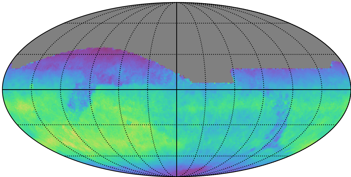
ddf_acor_sf10_lsf15_lsr10_v3.4_10yrs All sky z band: Normalized Teff
