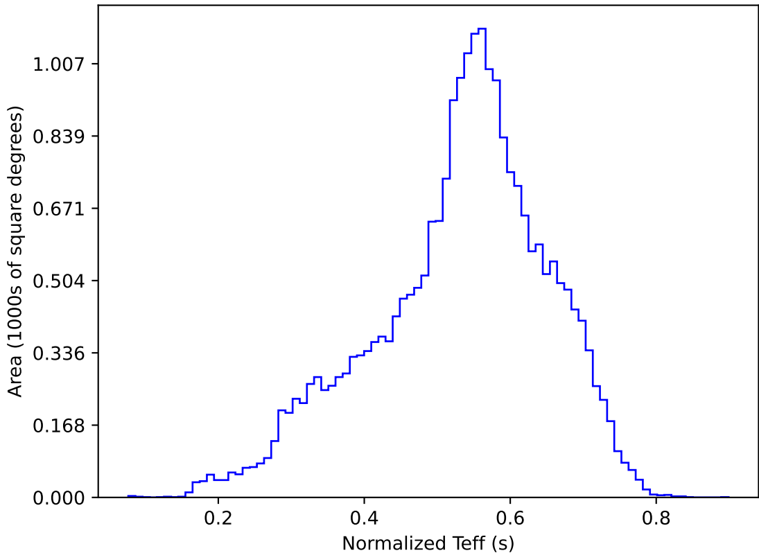
ddf_acor_sf10_lsf15_lsr10_v3.4_10yrs All sky y band: Normalized Teff
