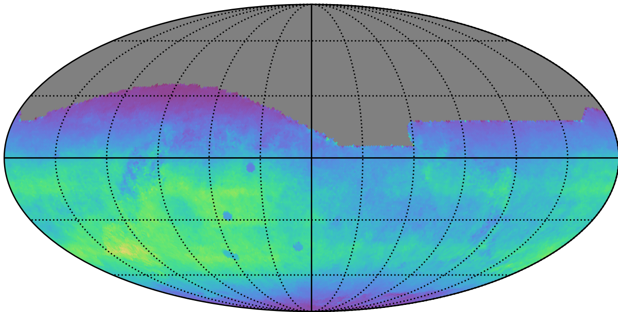
ddf_acor_sf10_lsf15_lsr10_v3.4_10yrs All sky r band: Normalized Teff
