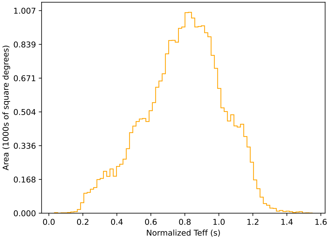
ddf_acor_sf10_lsf15_lsr10_v3.4_10yrs All sky r band: Normalized Teff
