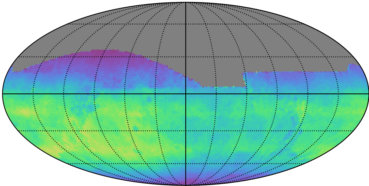
ddf_acor_sf10_lsf15_lsr10_v3.4_10yrs All sky i band: Normalized Teff
