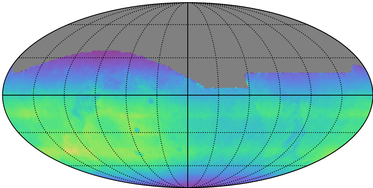
ddf_acor_sf10_lsf15_lsr10_v3.4_10yrs All sky all bands: Normalized Teff
