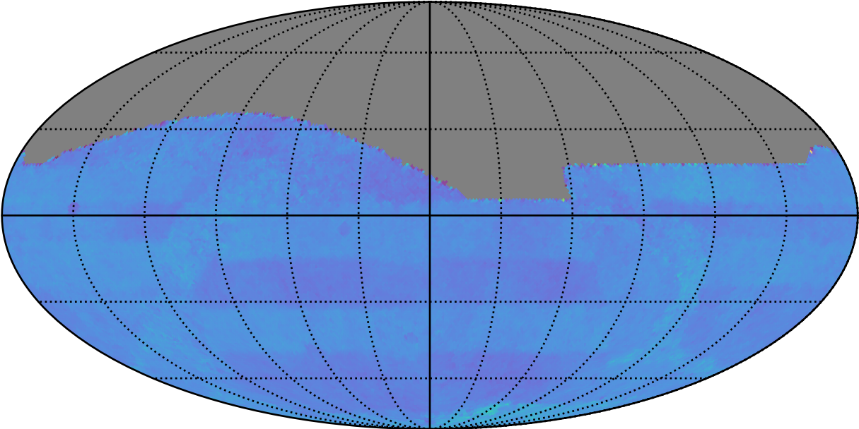
ddf_acor_sf10_lsf15_lsr10_v3.4_10yrs All sky: Normalized Proper Motion Uncert @ 24.0
