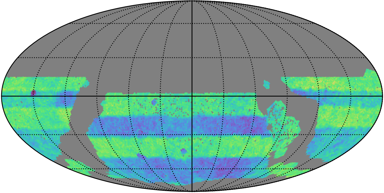
ddf_acor_sf10_lsf15_lsr10_v3.4_10yrs WFD: Normalized Proper Motion Uncert @ 20.5
