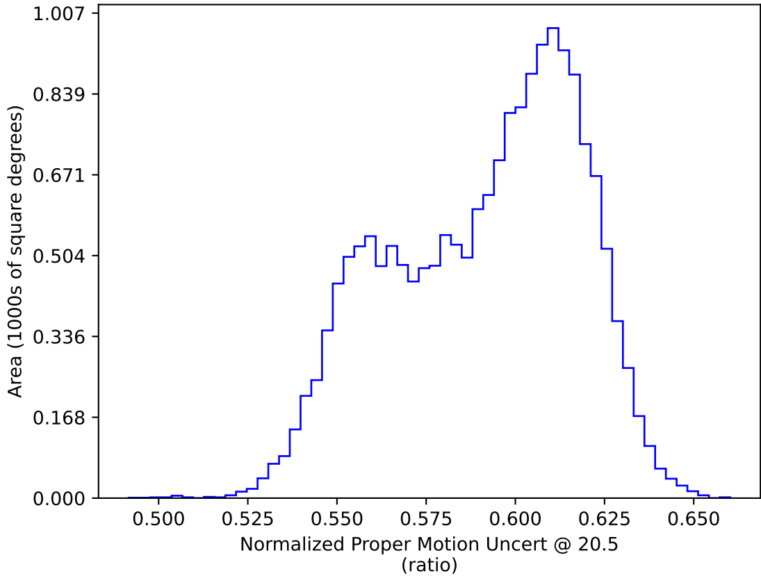
ddf_acor_sf10_lsf15_lsr10_v3.4_10yrs WFD: Normalized Proper Motion Uncert @ 20.5
