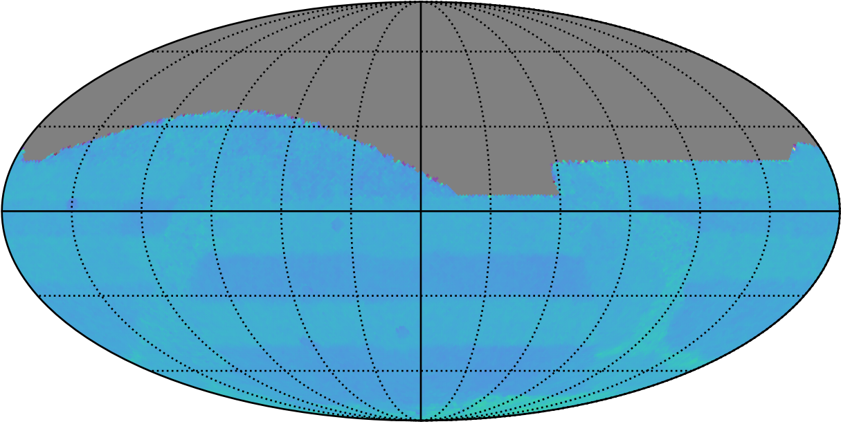
ddf_acor_sf10_lsf15_lsr10_v3.4_10yrs All sky: Normalized Proper Motion Uncert @ 20.5
