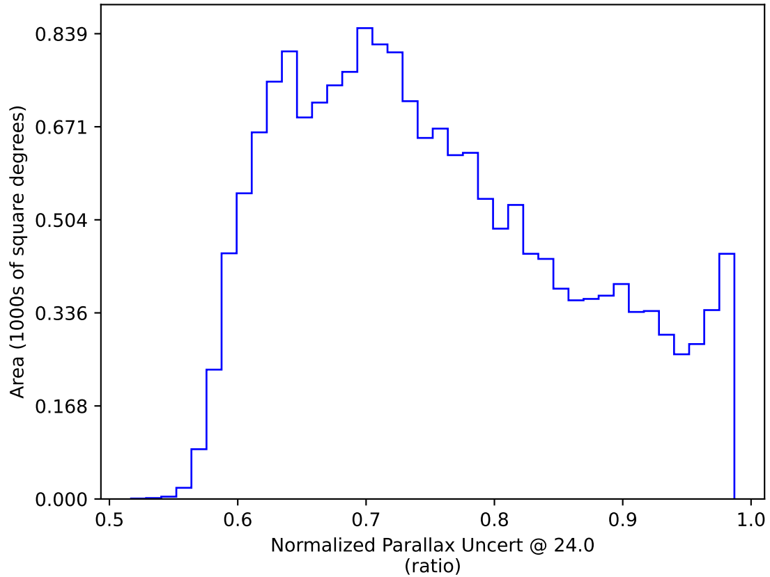
ddf_acor_sf10_lsf15_lsr10_v3.4_10yrs WFD: Normalized Parallax Uncert @ 24.0
