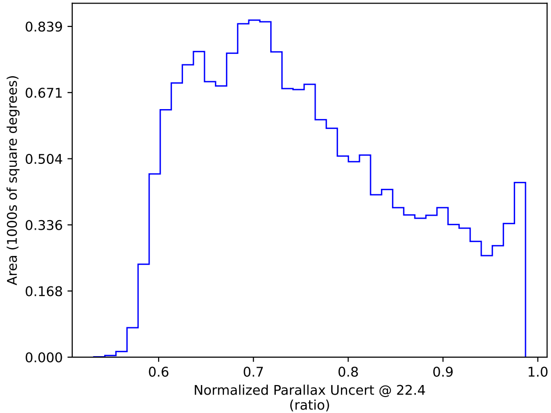
ddf_acor_sf10_ls15_lsr10_v3.4_10yrs WFD: Normalized Parallax Uncert @ 22.4
