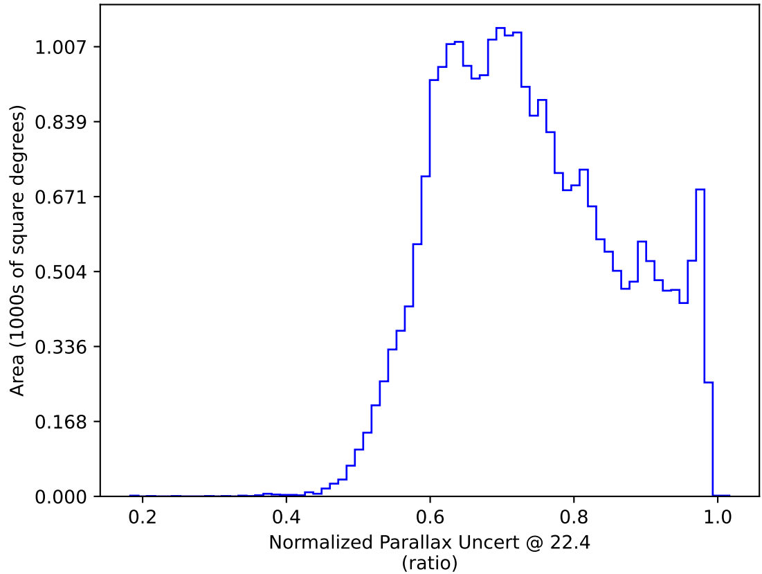
ddf_acor_sf10_lsf15_lsr10_v3.4_10yrs All sky: Normalized Parallax Uncert @ 22.4
