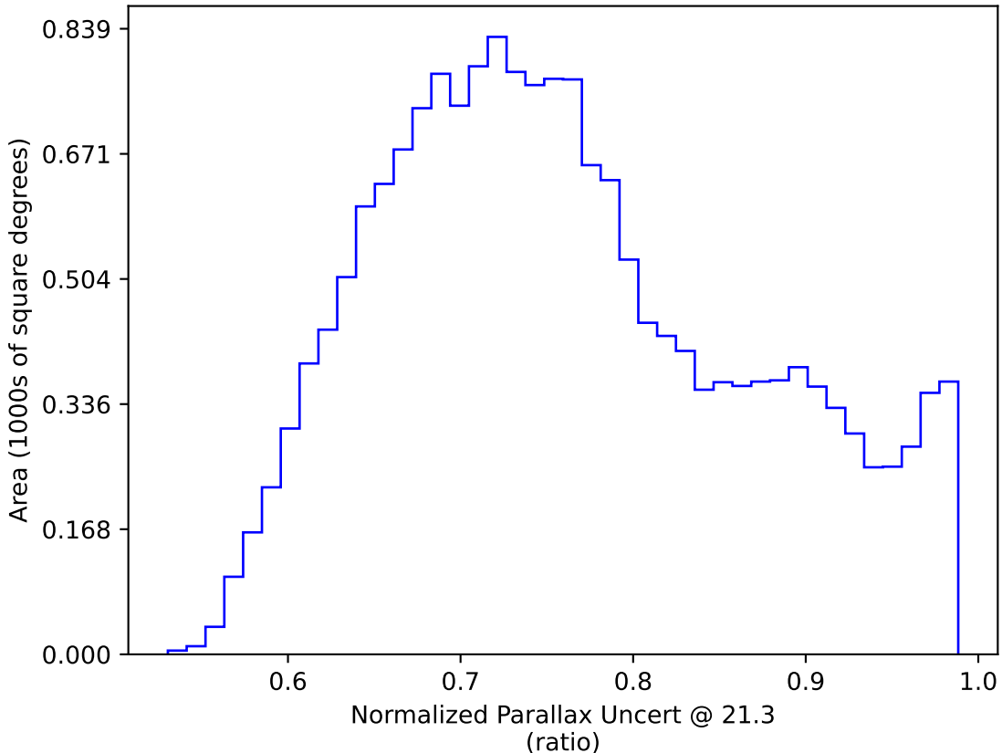
ddf_acor_sf10_lsf15_lsr10_v3.4_10yrs WFD y band only: Normalized Parallax Uncert @ 21.3
