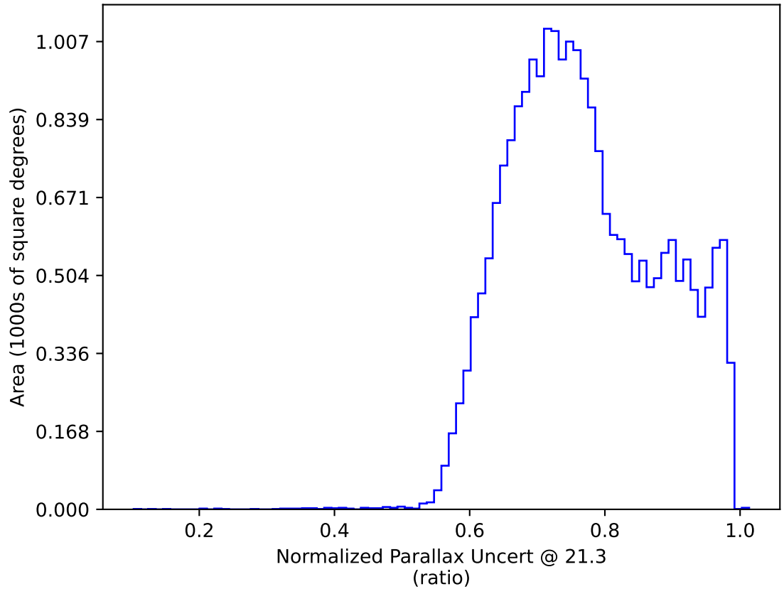
ddf_acor_sf10_lsf15_lsr10_v3.4_10yrs All sky y band only: Normalized Parallax Uncert @ 21.3
