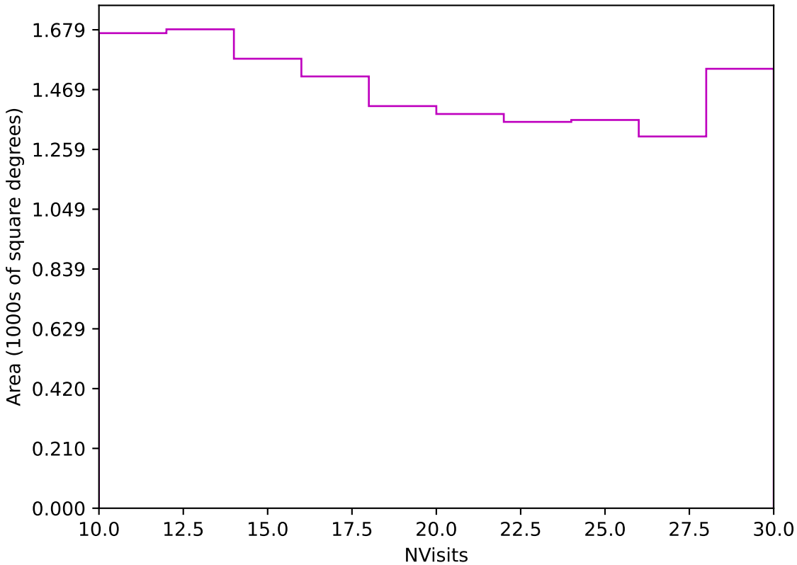
ddf_acor_sf10_lsf15_lsr10_v3.4_10yrs Yr 3-4 z band: NVisits
