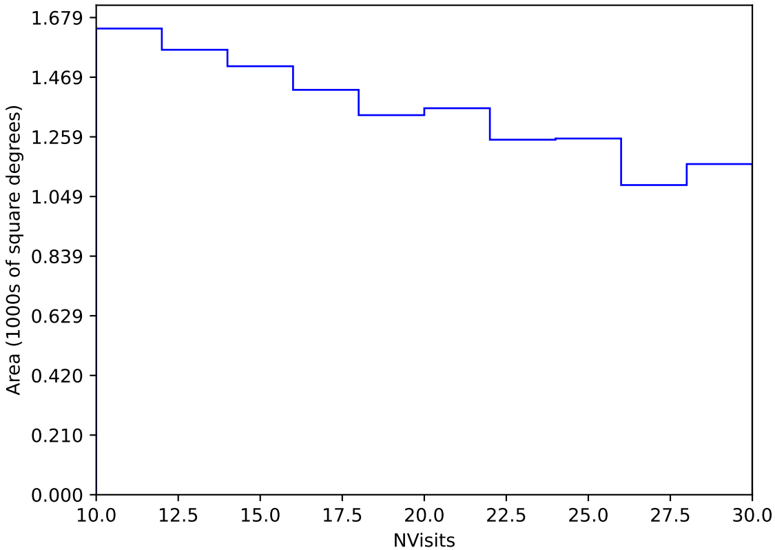
ddf_acor_sf10_lsf15_lsr10_v3.4_10yrs Yr 3-4 y band: NVisits
