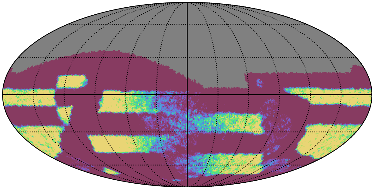
ddf_acor_sf10_lsf15_lsr10_v3.4_10yrs Yr 3-4 all bands: NVisits
