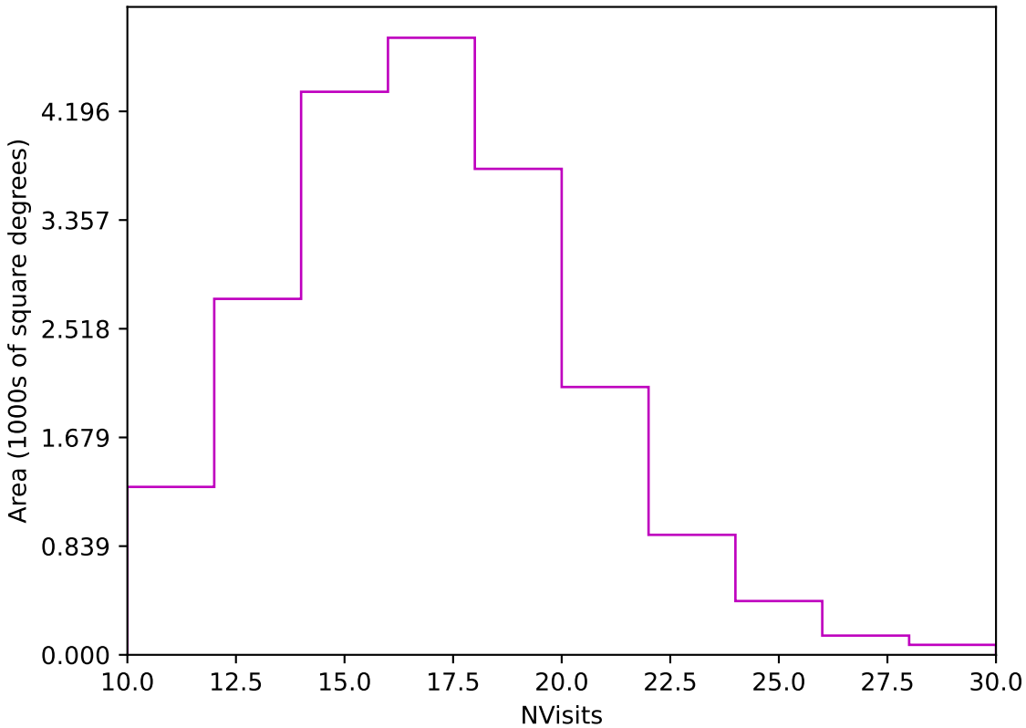
ddf_acor_sf10_lsf15_lsr10_v3.4_10yrs Yr 1 z band: NVisits
