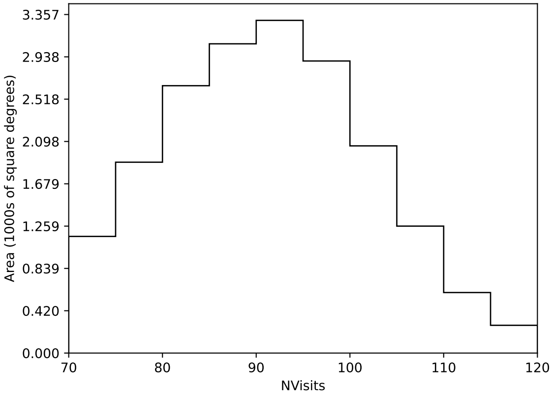
ddf_acor_sf10_lsf15_lsr10_v3.4_10yrs Yr 1 all bands: NVisits
