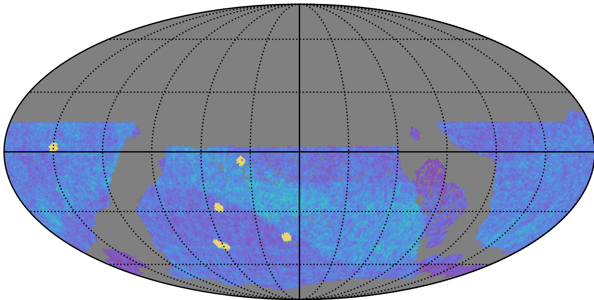
ddf_acor_sf10_lsf15_lsr10_v3.4_10yrs WFD z band: NVisits
