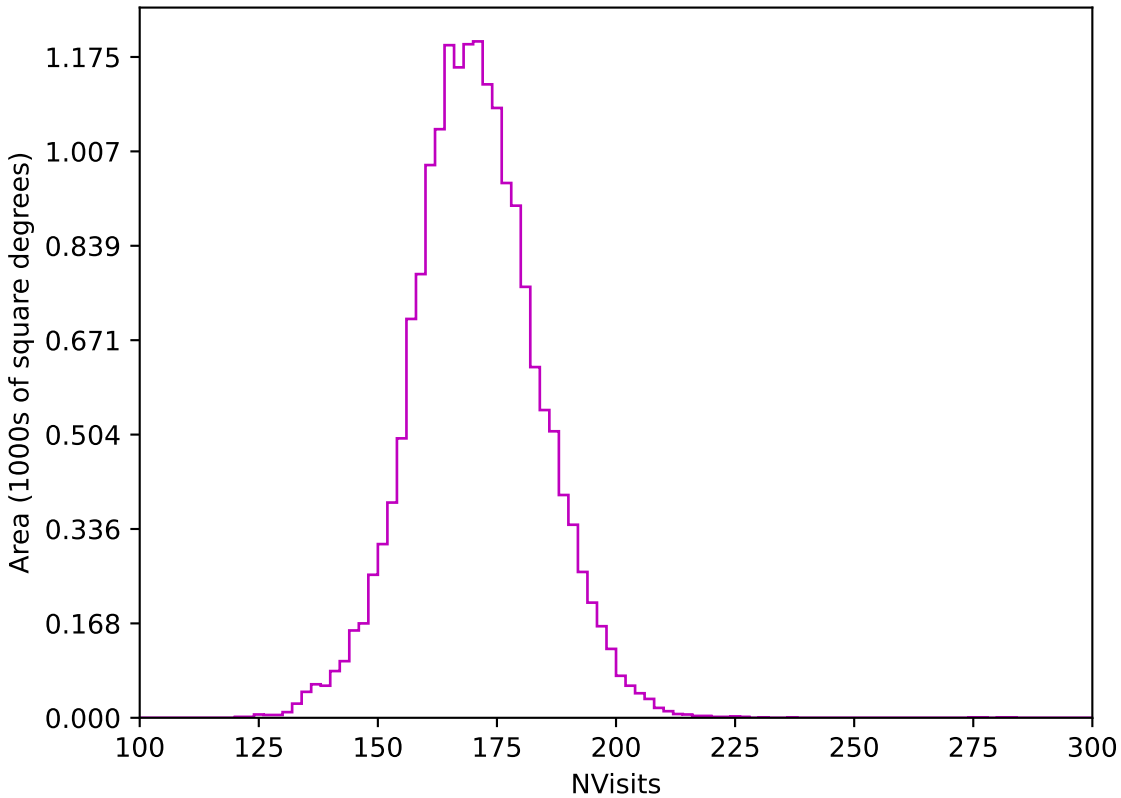
ddf_acor_sf10_lsf15_lsr10_v3.4_10yrs WFD z band: NVisits
